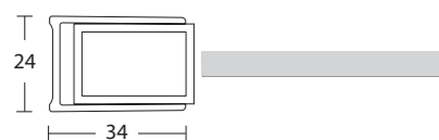
Art. 1125 profilé mural + Art. 1161 montant vertical Art. 1125 wall profile + art. 1161 vertical profile pour/for VO-PSO - VB-PSO - VA-PSO
