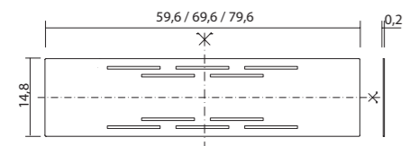
Grille couvre-bonde double face, en acier inox Stainless steel waste cover
