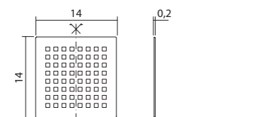
Grille couvre-bonde double face, en acier inox Stainless steel waste cover
