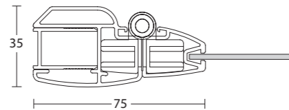
Art. 106 profilé mural + Art. 105 montant vertical + Art. 104 profilé vertical / charnière Art. 106 wall profile + Art. 105 vertical profile + Art. 104 vertical pivoting profile pour/for CO : SVM - 1PPI - 2PPI - 3PPI
