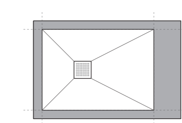
Section du receveur Arturo sans bords Position and size of the cut area for Arturo tray
